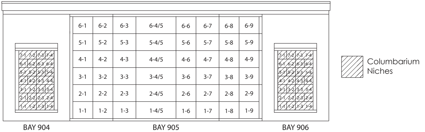
NORTH ELEVATION
